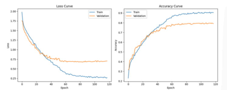
Figure 5 - Training and Validation Loss/Accuracy (SER CNN-BiLSTM)
