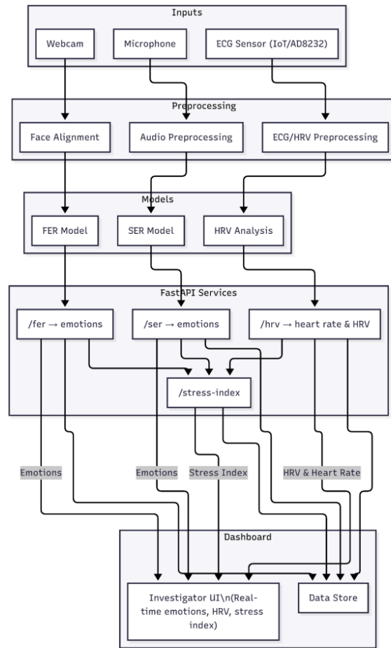
Figure 5 : Component Diagram Multimodal Behaviour & Emotional Analysis
